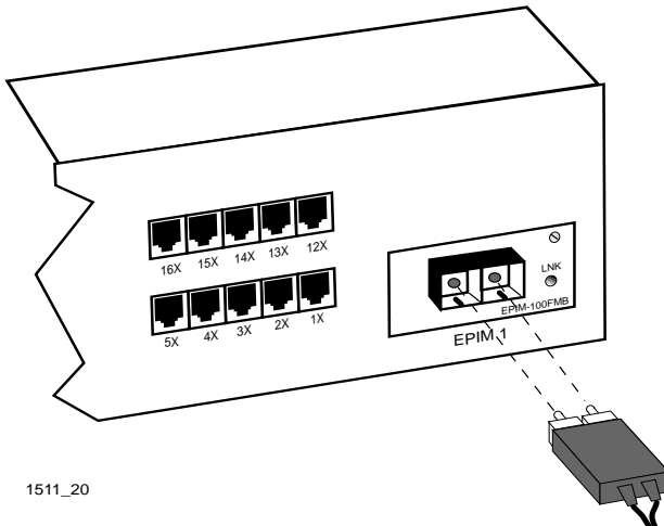
Figure A-3 EPIM-100FMB
